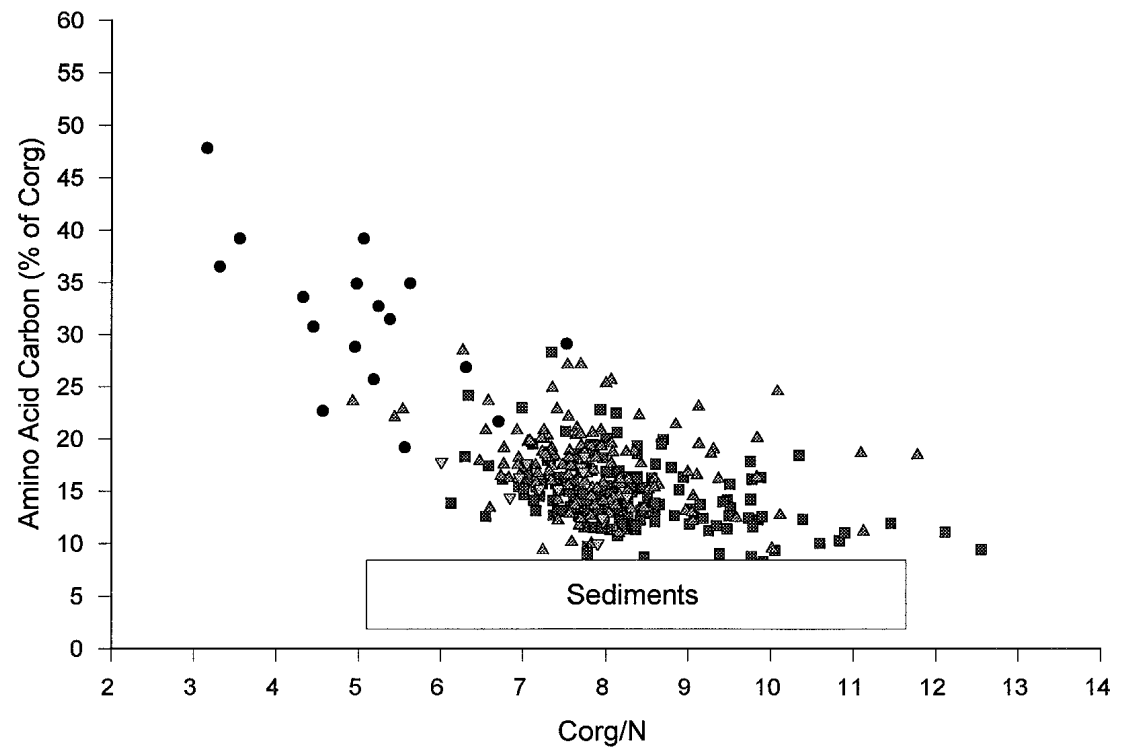
Figure 14.8 Amino acid carbon as per cent of organic carbon ( C_{org} ) versus C/N ratio in plankton (dots), shallow (triangles) and deep traps (squares) from the Arabian Sea, and in sediments from the Arabian Sea (box).
