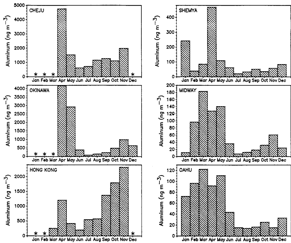
Figure 3.4 Monthly mean Al aerosol concentrations in the North Pacific PEM-West network (Arimoto et al., 1995b).
