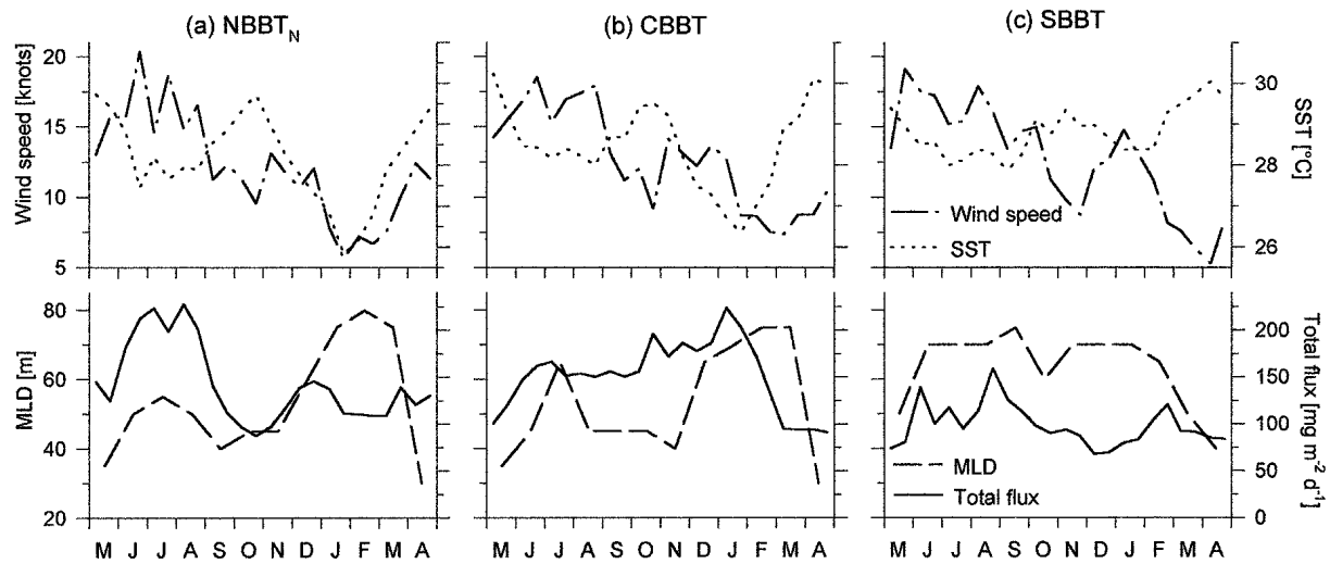
Figure 15.6 Biweekly means of wind speed, sea surface temperature (SST), mixed layer depth (MLD, from Rao et al., 1989) and total flux in the (a) northern, (b) central and (c) southern Bay of Bengal.
